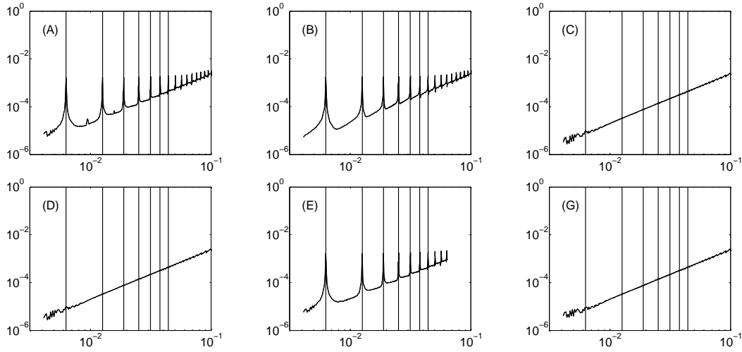
Figure 2. Global error in positions at t = 1 of the methods versus step size
