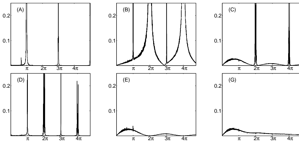
Figure 1. Maximum error of total energy on the interval [0, 1000] as a function of h\omega (step size h = 0.02 ).
