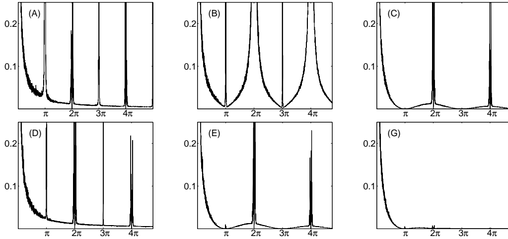
Figure 3. Maximum deviation of the oscillatory energy on the interval [0, 1000] as a function of h\omega (step size h = 0.02 ).
